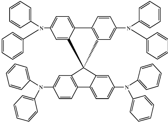
spiro-TPD
