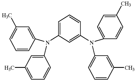
PDA
