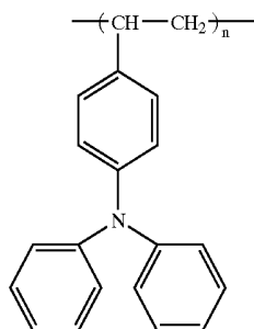
DPA-PS
