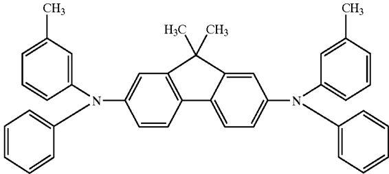
DTDPFL
